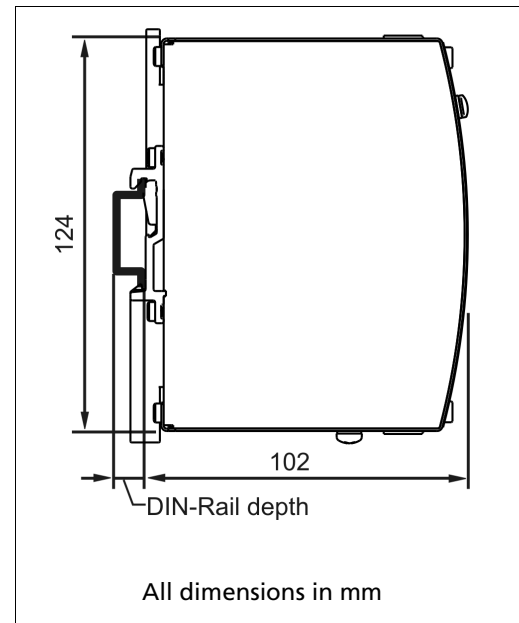
Fig. 21-2 Side view
