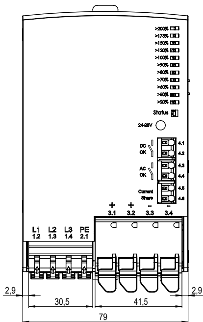
Fig. 27-1: Front view
