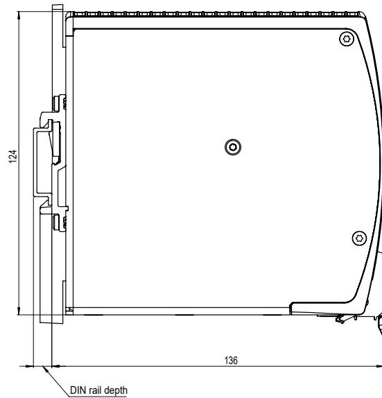
Fig. 27-2: Side view
