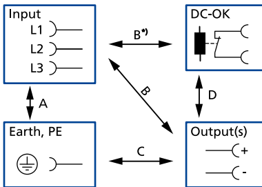
Fig. 24-1: Dielectric strength
