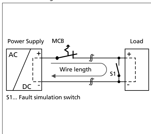
Fig. 23-5 Test circuit
