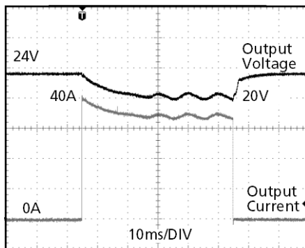
Peak load 40A (resistive) for 50ms Output voltage dips from 24V to 20V.
