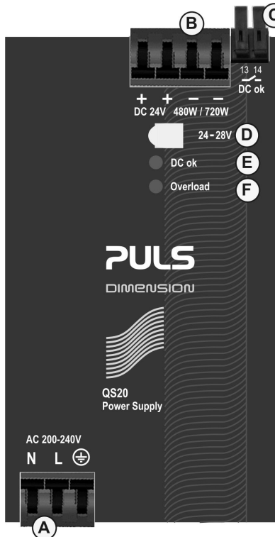
Fig. 13-1 Front side
