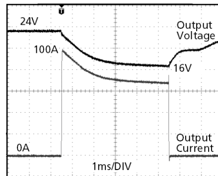
Peak load 100A (resistive) for 5ms Output voltage dips from 24V to 16V.
