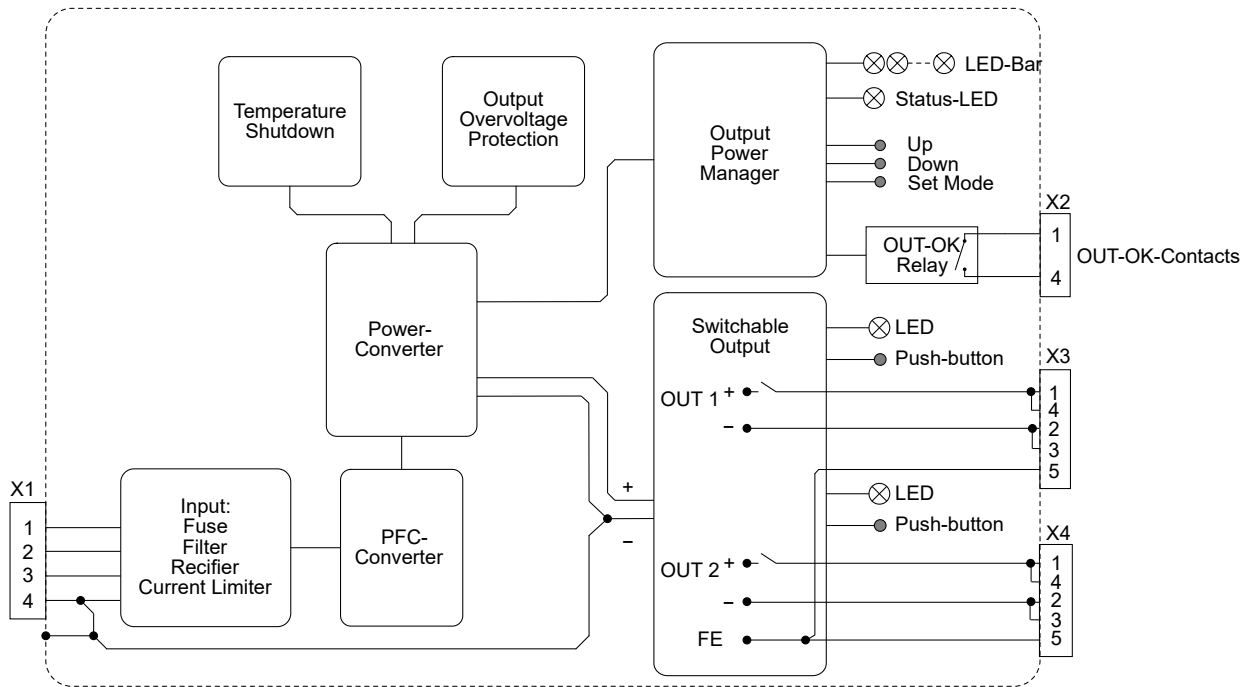
Fig. 12-1: Functional Diagram FPT500.245-034-106
