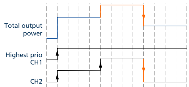
Fig. 6-2: Tripping of the channel with the lowest priority when the power budget is exceeded
