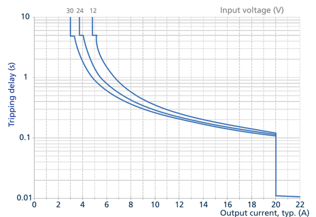
Fig. 6-2: Tripping delay depending on input voltage slow tripping characteristic
