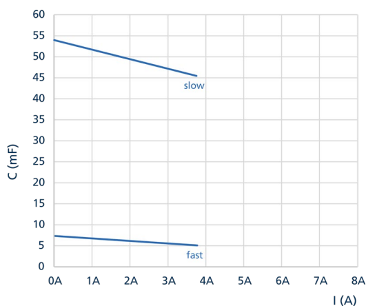
Fig. 7-1: Typical capacitive loads for slow/fast tripping characteristic at 24V
