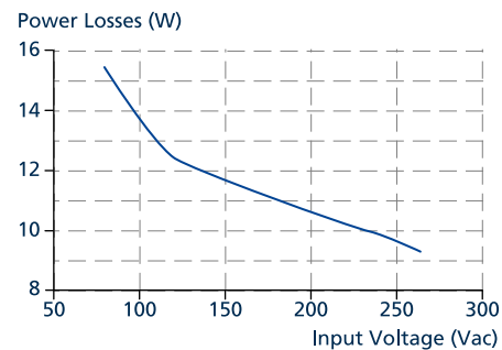
Fig. 9-4: Losses vs. input voltage at 24 V, 188 W, typ.
