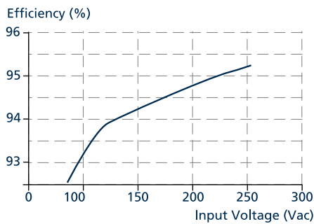
Fig. 9-3: Efficiency vs. input voltage at 24 V, 188 W, typ.
