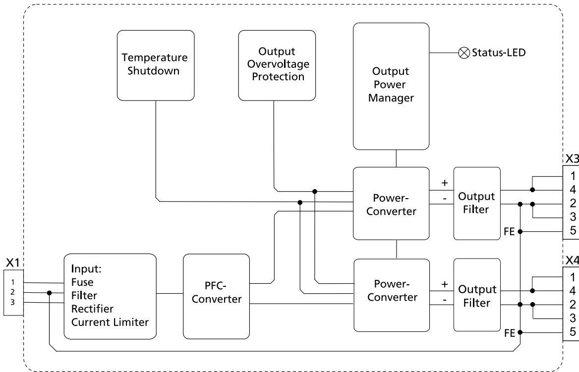
Fig. 12-1: Functional Diagram FPS202.241-003
