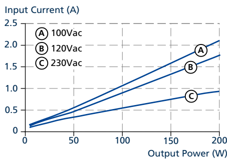
Fig. 4-3: Input current vs. output power at 24 V output voltage
