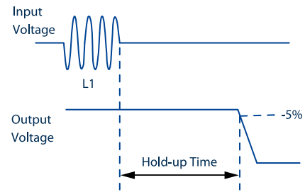
Fig. 8-2: Shut-down behavior, definitions
