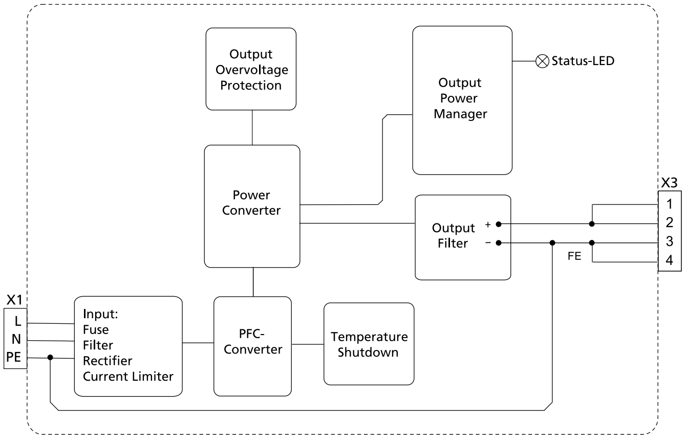
Fig. 12-1: Functional Diagram FPS100.241-009
