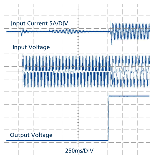
Fig. 6-1: Typical turn-on behavior at nominal load and +25 °C ambient temperature
