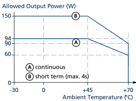
Fig. 16-1: Output power vs. ambient temp.
