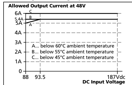
Fig. 4-2 Derating requirements
