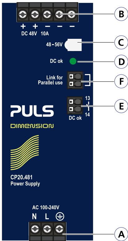
Fig. 14-1: Front side
