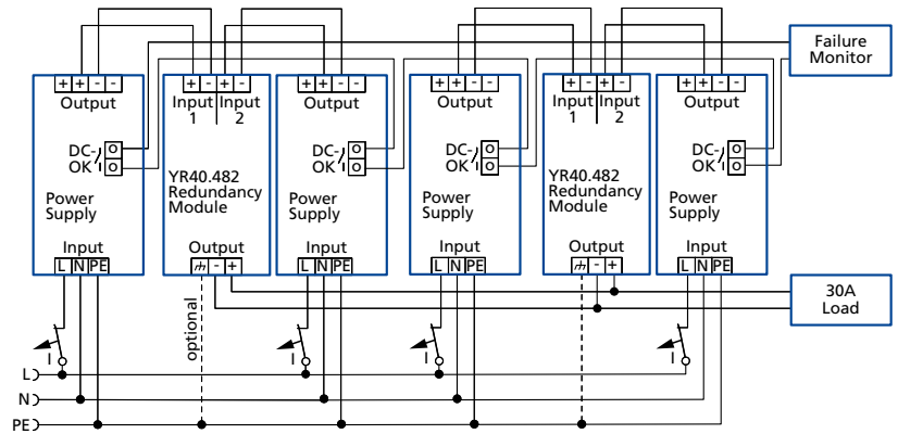
Fig. 24-6: N+1 Redundant configuration for 30A load current with multiple devices and redundancy modules
