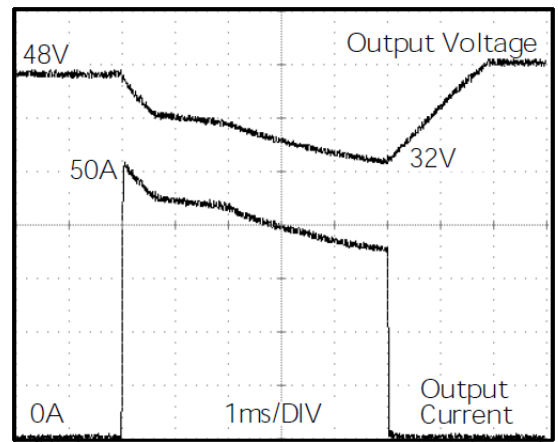
Fig. 24-2: 50A peak current for 5ms , typ. (5x the nominal current)
