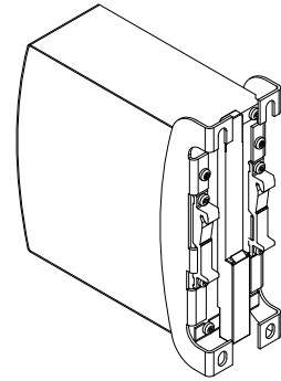
Fig. 23-3: Isometric view
