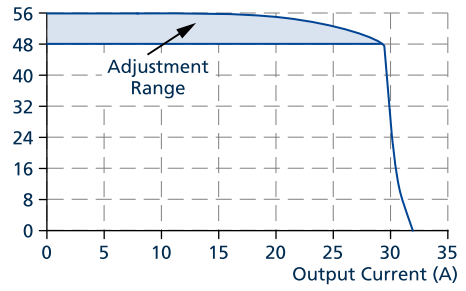
Fig. 6-2: Dynamic overcurrent capability, typ.
