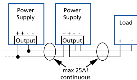
Fig. 13-1: Daisy chaining of outputs
