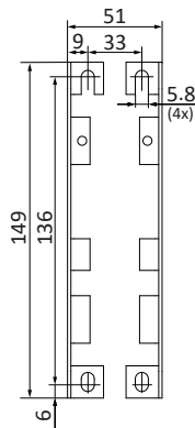
Fig. 23-5: Hole pattern for wall mounting
