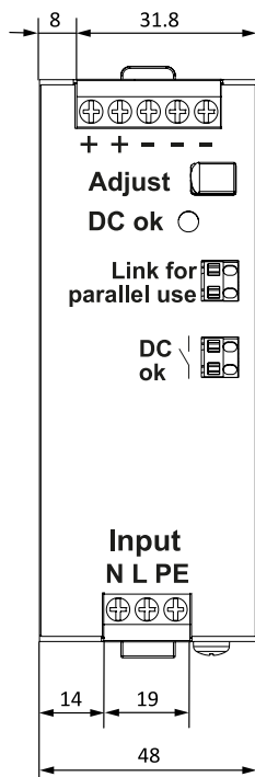
Fig. 22-1: Front view
