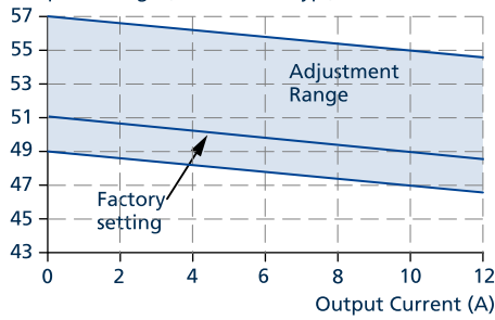
Fig. 6-4: Output voltage in "parallel use" mode, typ.
