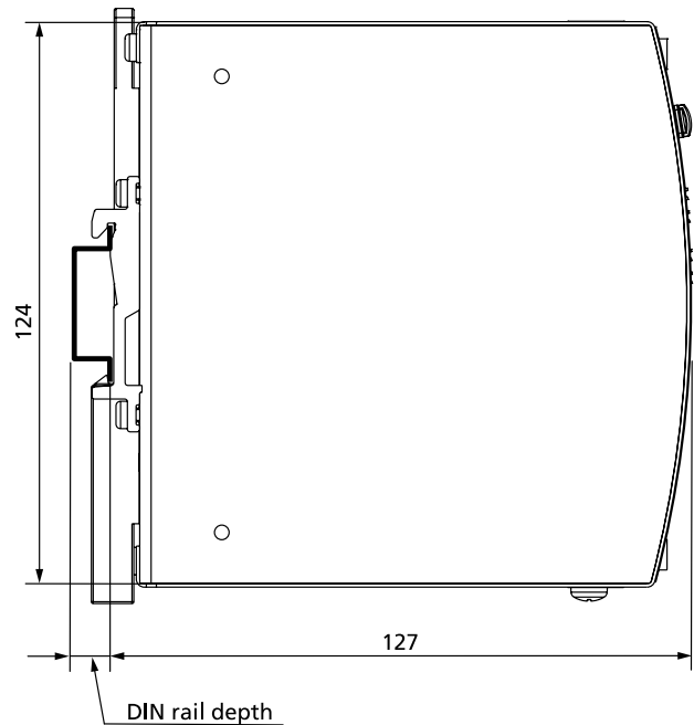
Fig. 22-2: Side view
