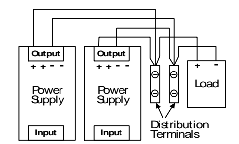
Fig. 22-6 Using distribution terminals
