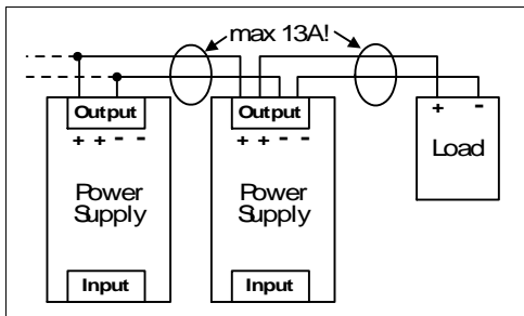
Fig. 22-5 Daisy chaining of outputs
