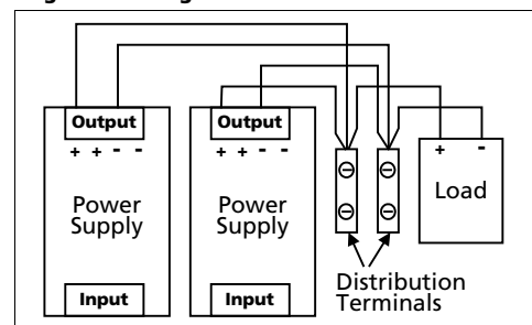
Fig. 22-6 Using distribution terminals
