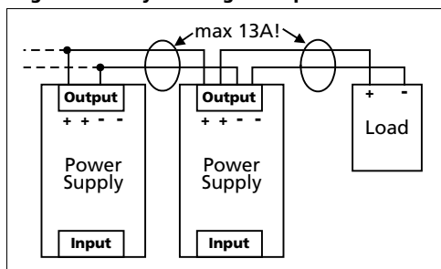
Fig. 22-5 Daisy chaining of outputs
