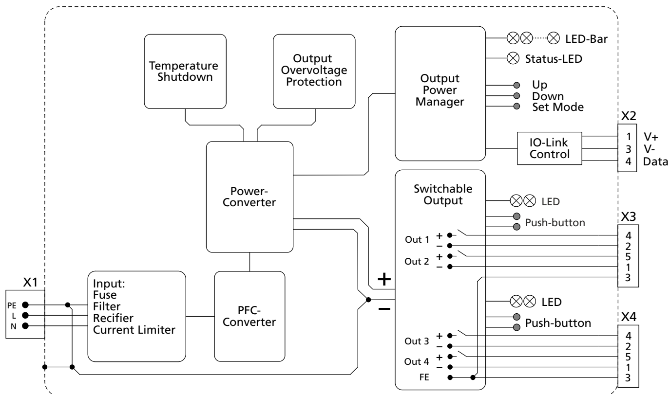
Fig. 12-1: Functional Diagram FPS300.245-055-109
