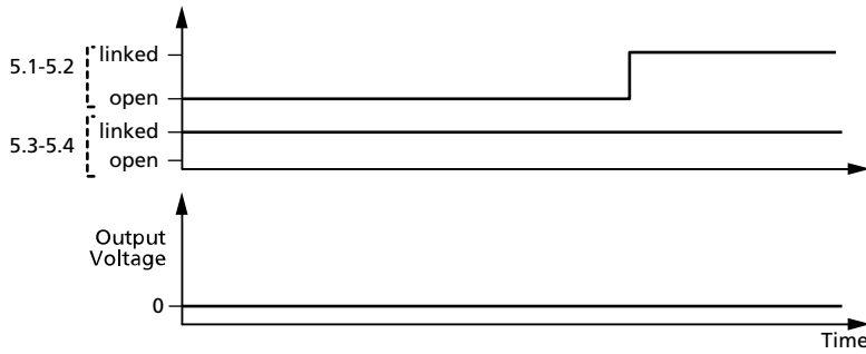
Fig. 12-3: Case 3: Pin 5.3 und Pin 5.4 linked, power supply OFF
