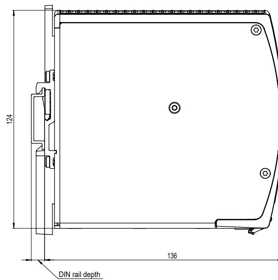
Fig. 28-2: Side view
