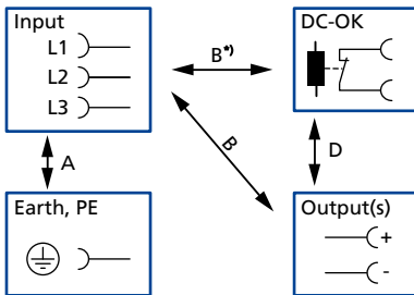
Fig. 25-1: Dielectric strength
