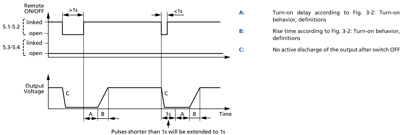
Fig. 12-1: Case 1: Pin 5.1 und Pin 5.2 linked, power supply on
