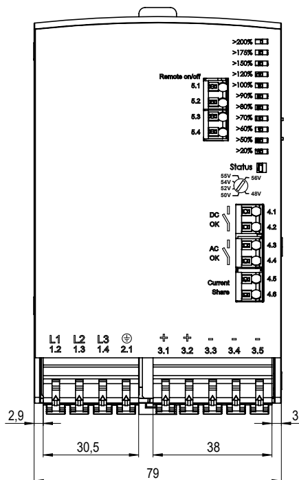
Fig. 28-1: Front view
