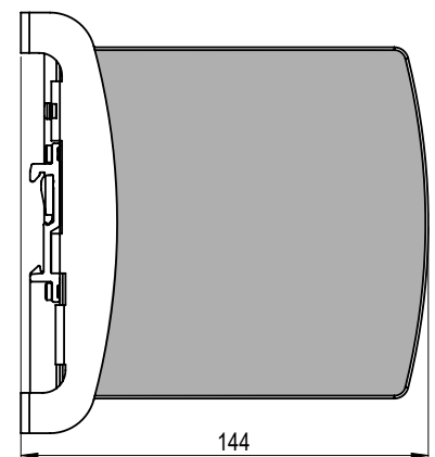
Fig. 29-6: Wall / panel mounting, side view
