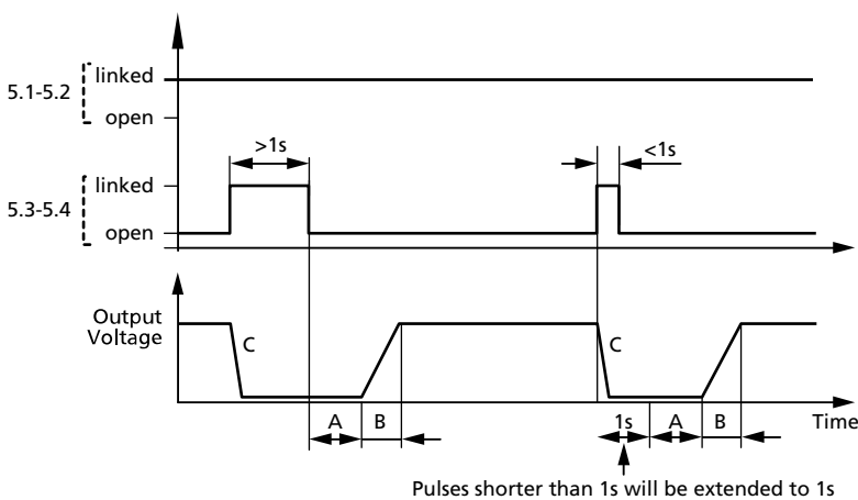
Fig. 12-2: Case 2: Pin 5.1 und Pin 5.2 linked, inverse behavior on Pin 5.3 and Pin 5.4
