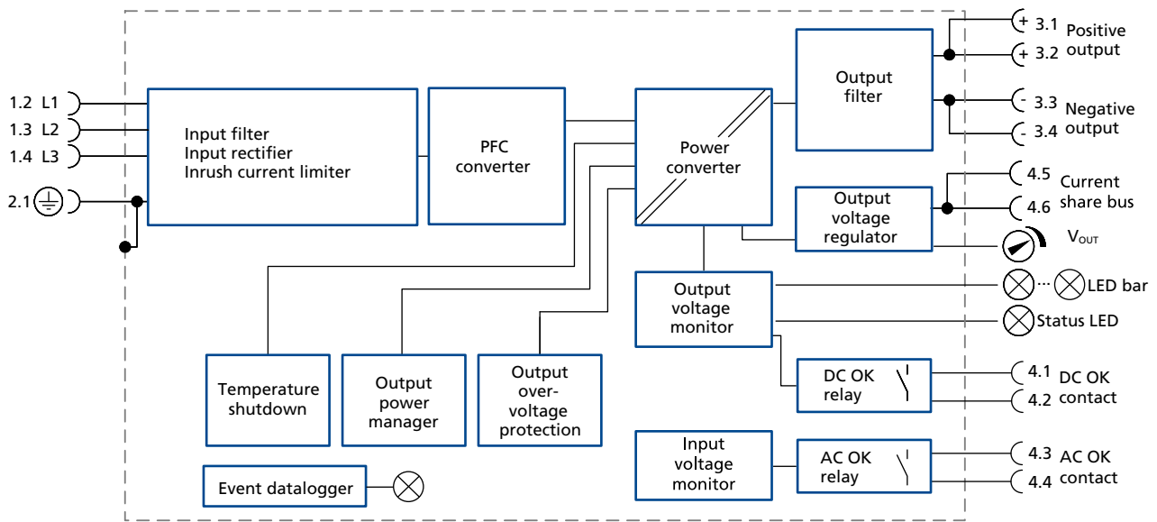
Fig. 17-1: Functional Diagram TP960.241
