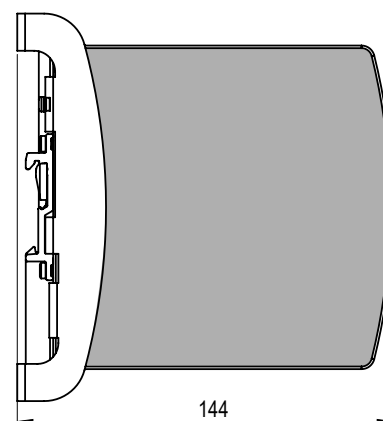
Fig. 29-6: Wall / panel mounting, side view
