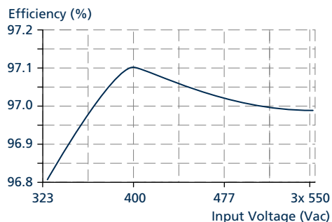
Fig. 14-3: Efficiency vs. input voltage at 24 V, 40 A, typ.
