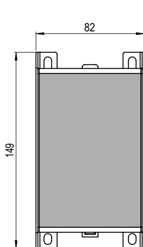
Fig. 29-4: Wall / panel mounting, front view
