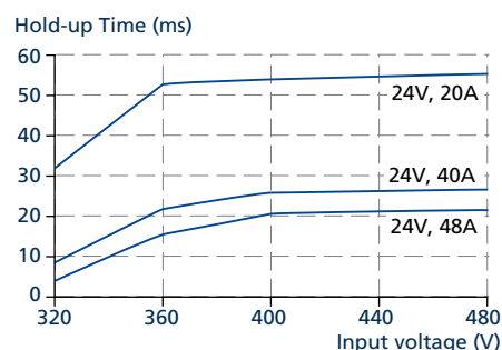
Fig. 30-2: Hold-up time vs. input voltage
