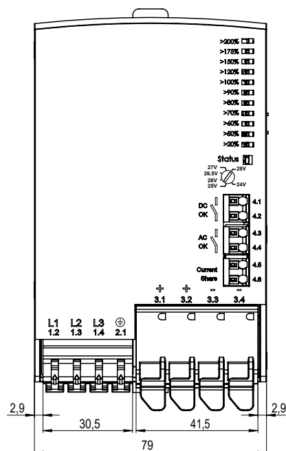
Fig. 28-1: Front view
