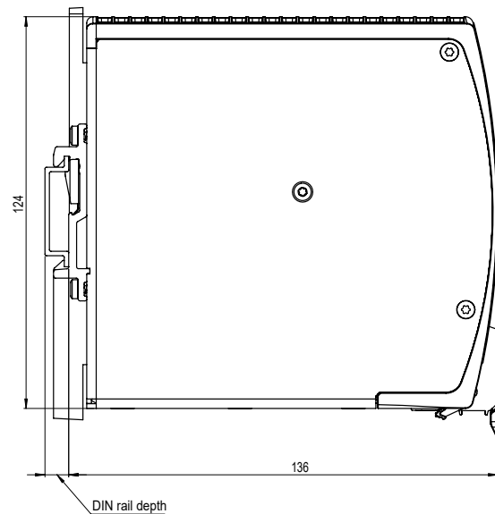
Fig. 28-2: Side view
