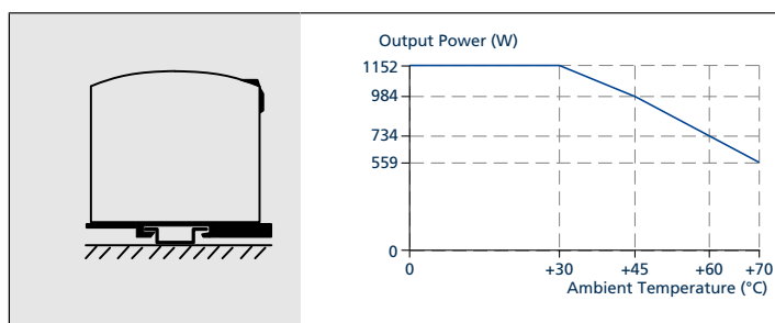
C Table-top mounting
