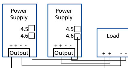
Fig. 18-3: Load with multiterminal
