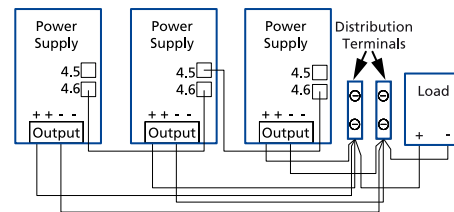
Fig. 18-2: Using distribution terminals
