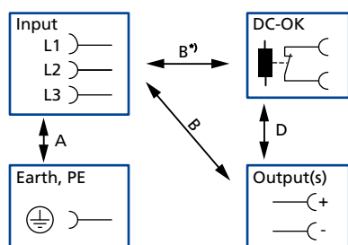
Fig. 25-1: Dielectric strength
