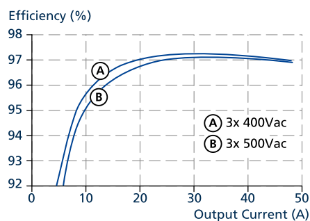
Fig. 14-1: Efficiency vs. output current at 24 V, typ.
