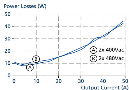
Fig. 30-4: Power Losses vs. output current at 24 V
