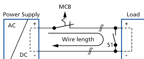
Fig. 30-5: Test circuit
