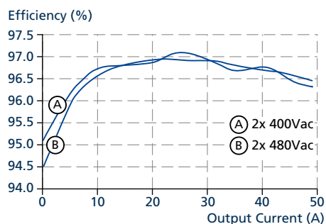
Fig. 30-3: Efficiency vs. output current at 24 V
