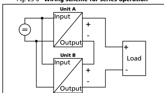
Fig. 23-6 Wiring scheme for series operation
