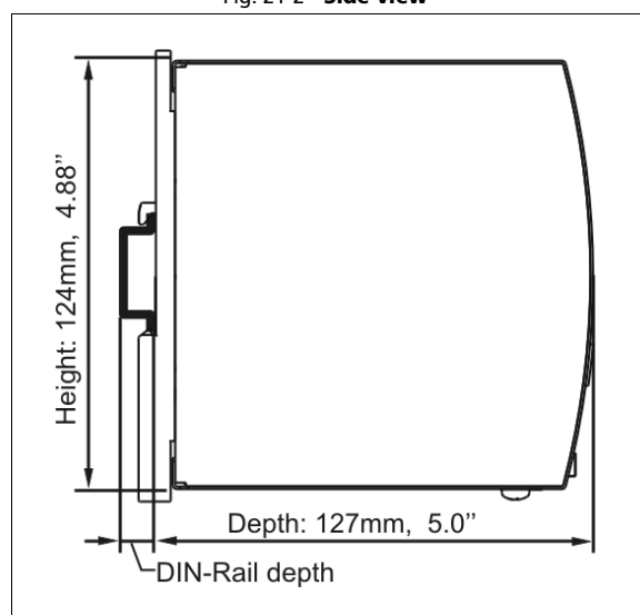
Fig. 21-2 Side view
