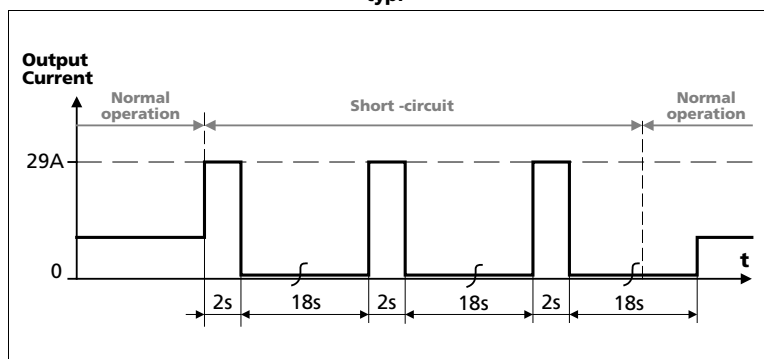
Fig. 6-2 Short-circuit on output, Hiccup PLUS mode, typ.
