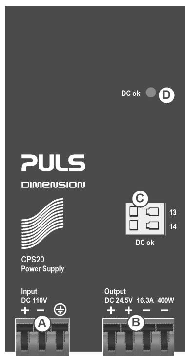
Fig. 13-1 Front side
