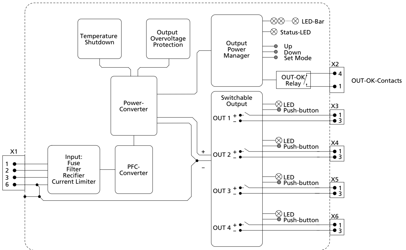
Fig. 12-1: Functional Diagram FPT300.246-042-101
