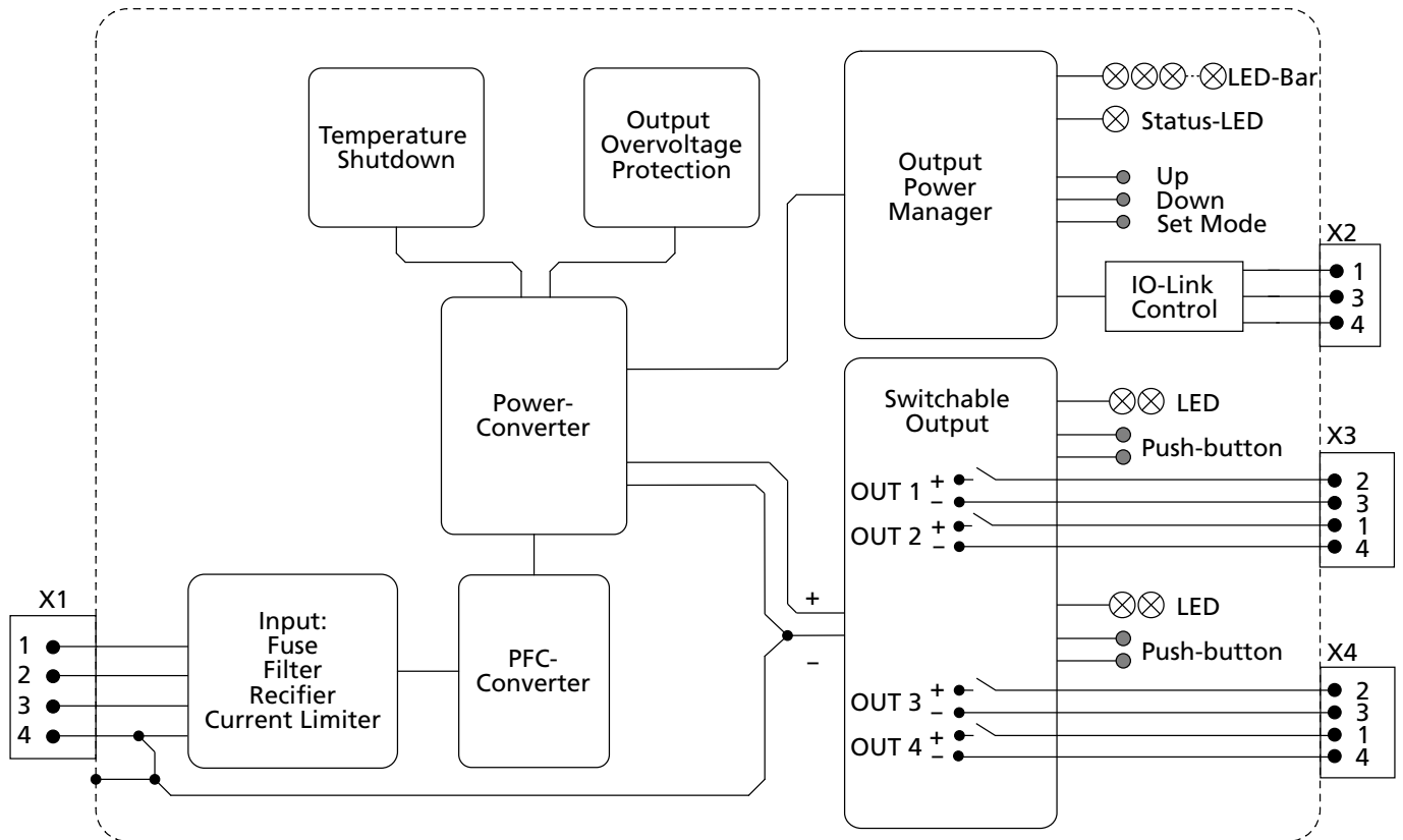
Fig. 12-1: Functional Diagram FPT500.245-018-103
