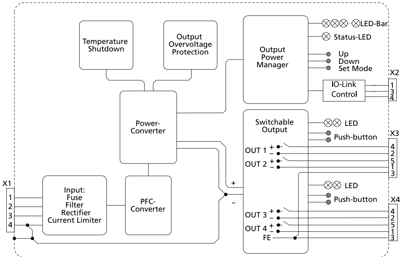
Fig. 12-1: Functional Diagram FPT500.245-062-117
