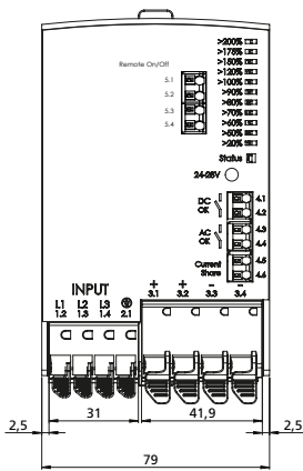
Fig. 28-1: Front view
