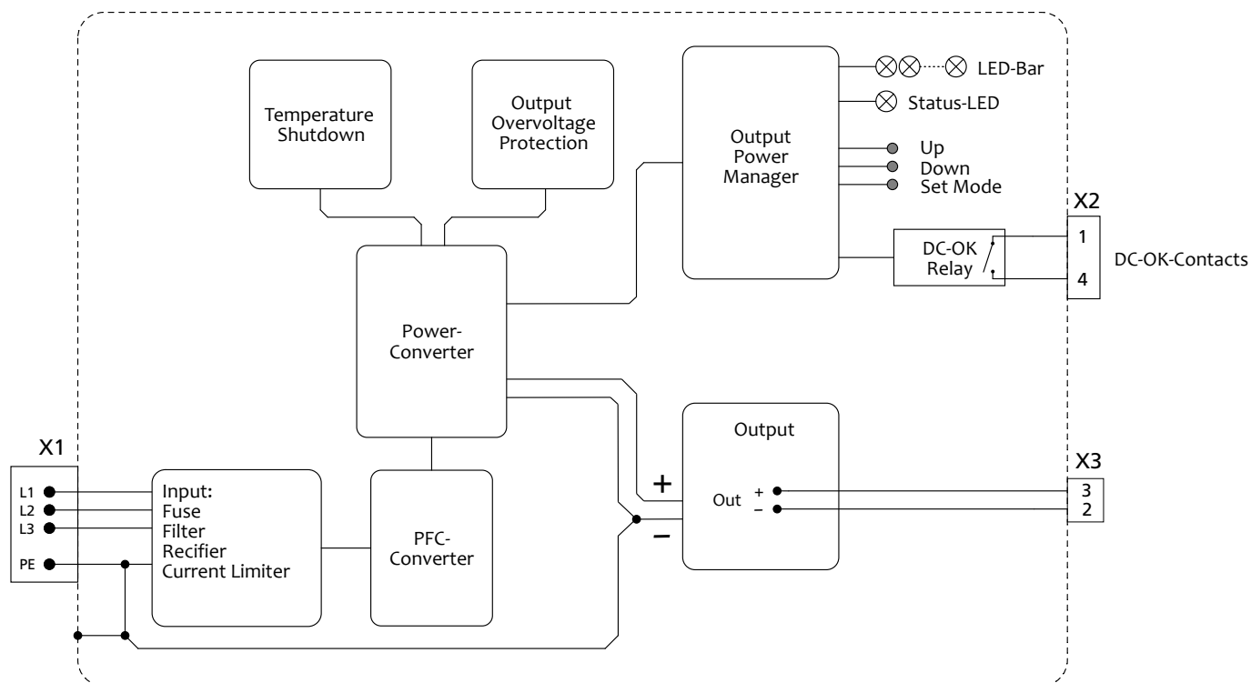
Fig. 12-1: Functional Diagram FPT500.481-002-101
