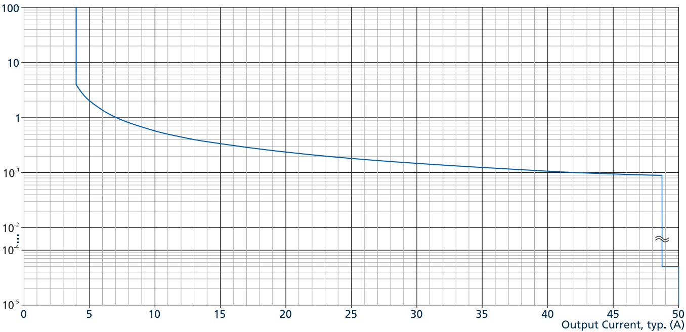
Fig. 6-2: Tripping curve diagram for NEC Class 2
