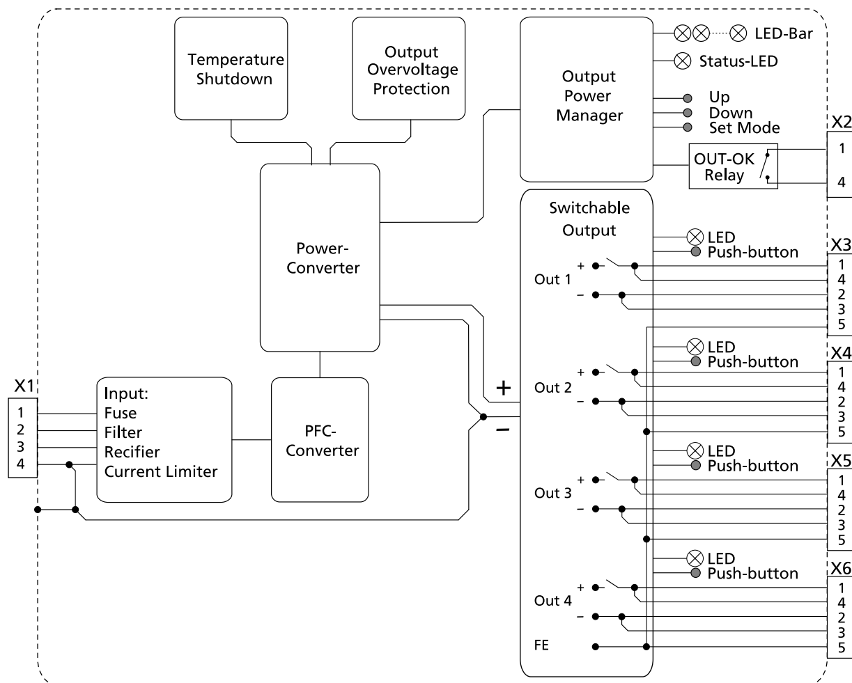
Fig. 12-1: Functional Diagram FPT300.246-065-103
