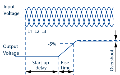
Fig. 3-2: Turn-on behaviour, definitions
