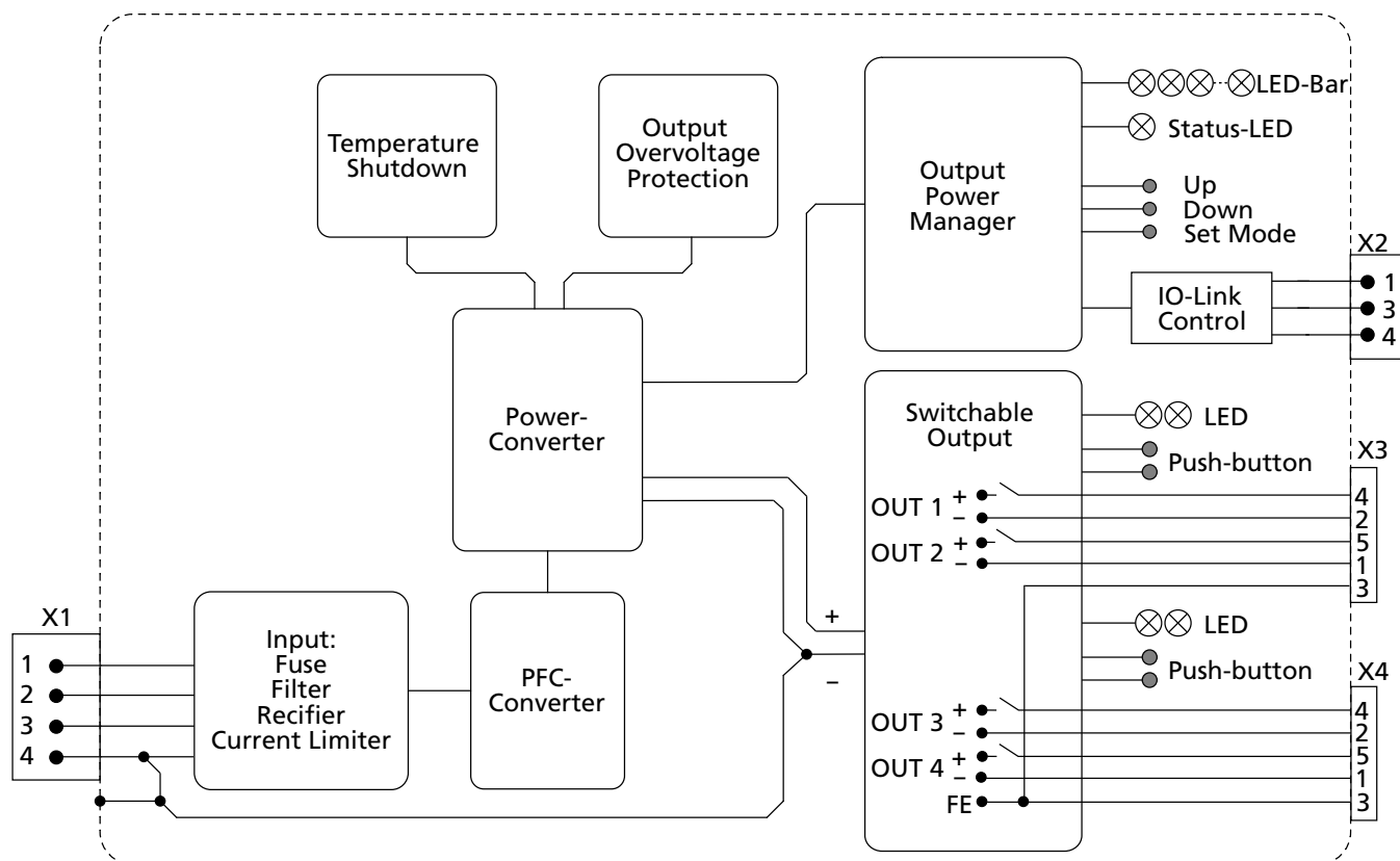
Fig. 12-1: Functional Diagram FPT500.245-055-158
