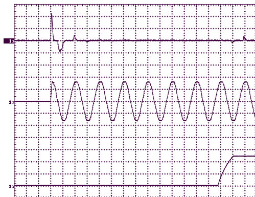
Fig. 5-1 Typical input inrush current behaviour
