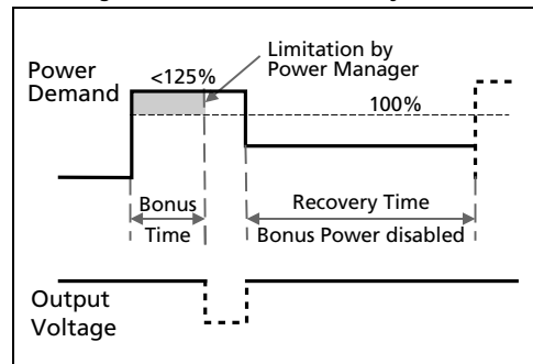
Fig. 5-4 BonusPower recovery time
