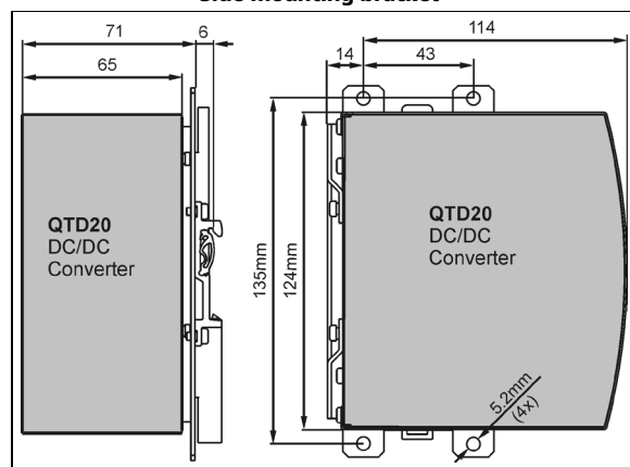
Fig. 22-6 Mounting Dimensions Side mounting bracket
