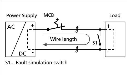
Fig. 23-5 Test circuit
