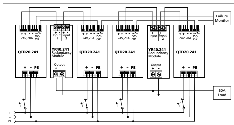
Fig. 22-8 Typical N+1 Redundant configuration for 60A with two dual redundancy modules and four DC/DC converters
