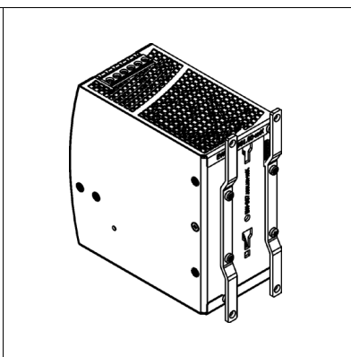
Fig. 22-2 Wall/panel mounting
