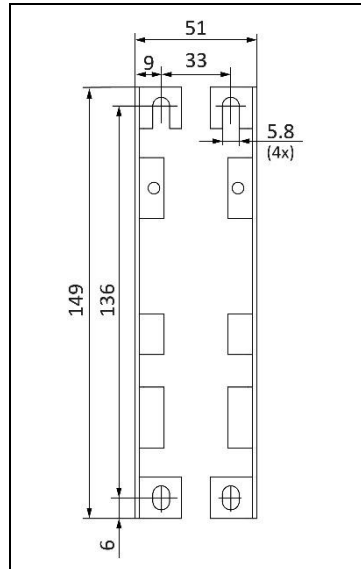
Fig. 25-5 Hole pattern for wall mounting
