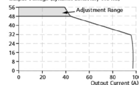
Output Voltage (dynamic behavior, <10 ms)
