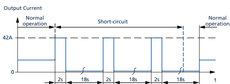
Fig. 6-2: Short-circuit on output, overcurrent mode, typ.
