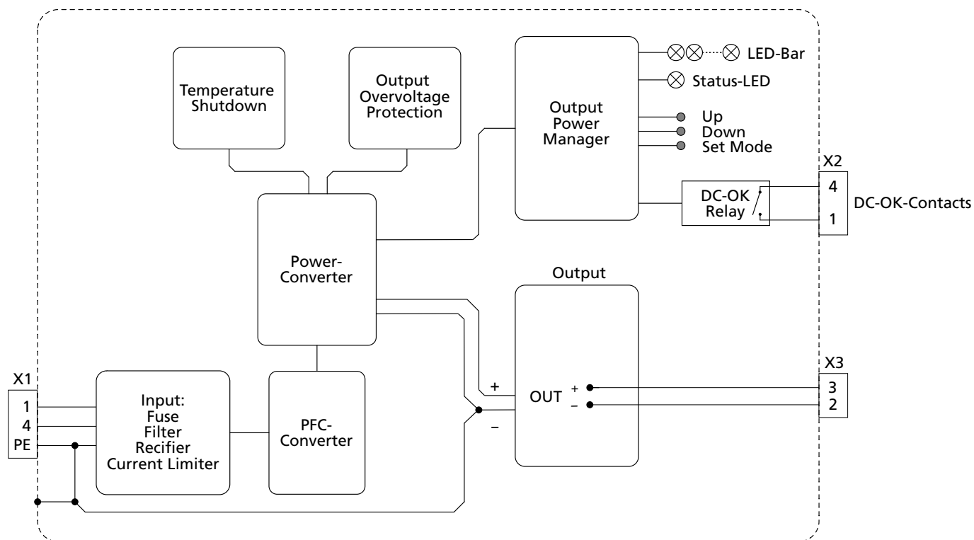
Fig. 12-1: Functional Diagram FPH500.241-002-101
