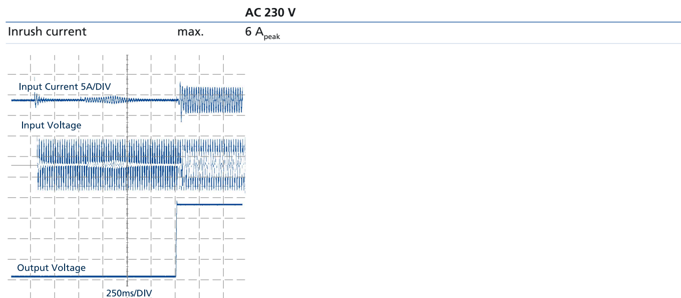
Fig. 5-1: Typical turn-on behavior at nominal load and +25 °C ambient temperature
