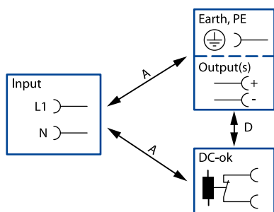
Fig. 18-1: Dielectric strength
