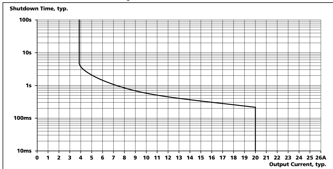
Fig. 6-1 Shutdown characteristic
