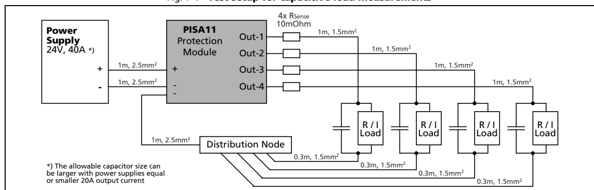
Fig. 7-1 Test setup for capacitive load measurements
