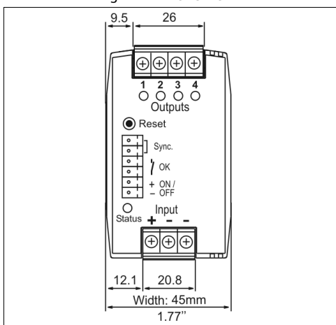
Fig. 24-1 Front view
