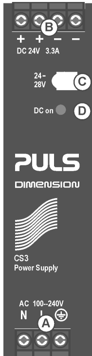
Fig. 12-1 Front side
