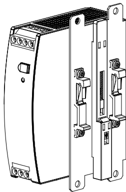
Side mounting with DIN rail brackets
