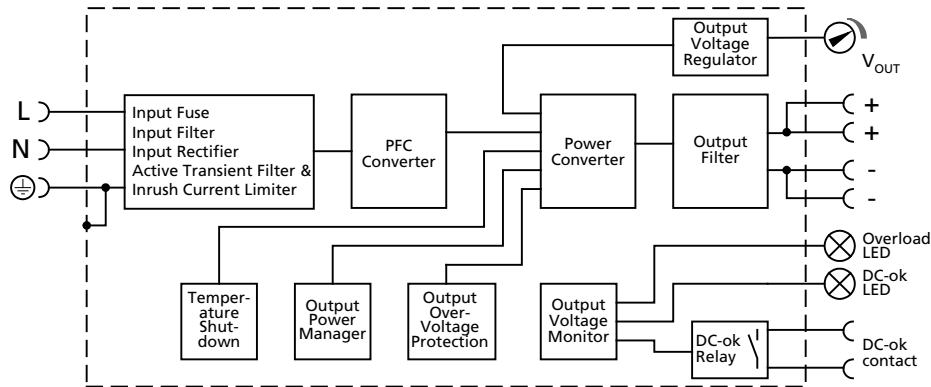
Fig. 11-1 Functional diagram
