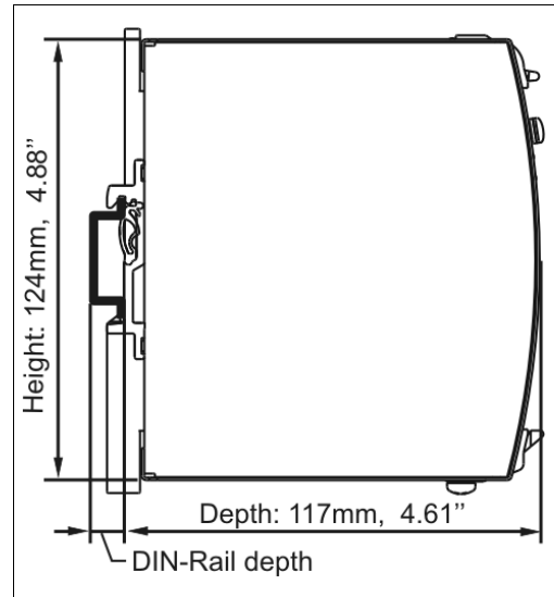
Fig. 21-2 Side view
