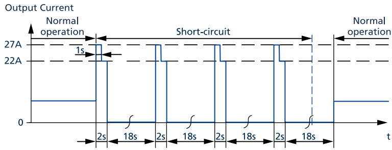
Fig. 6-3: Short term output current capability, typ.
