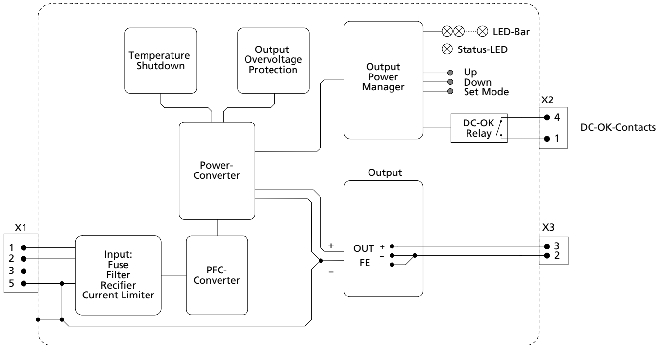
Fig. 12-1: Functional Diagram FPT300.242-002-101
