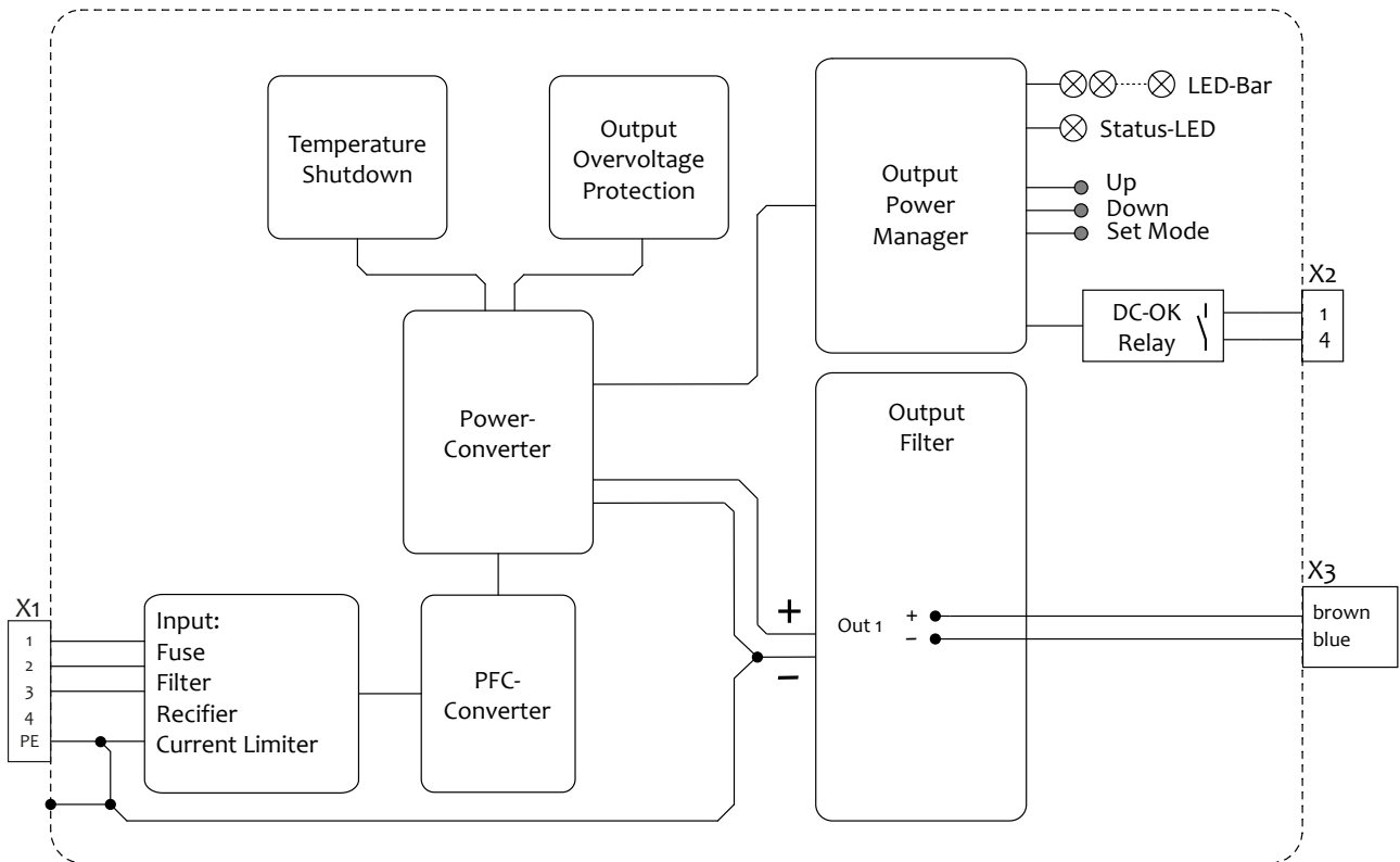
Fig. 12-1: Functional Diagram FPT500.481-008-103
