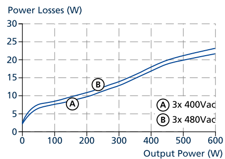
Fig. 9-2: Losses vs. output power at 48 V, typ.
