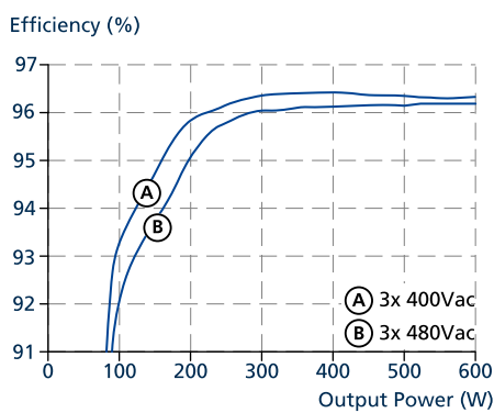
Fig. 9-1: Efficiency vs. output power at 48 V, typ.
