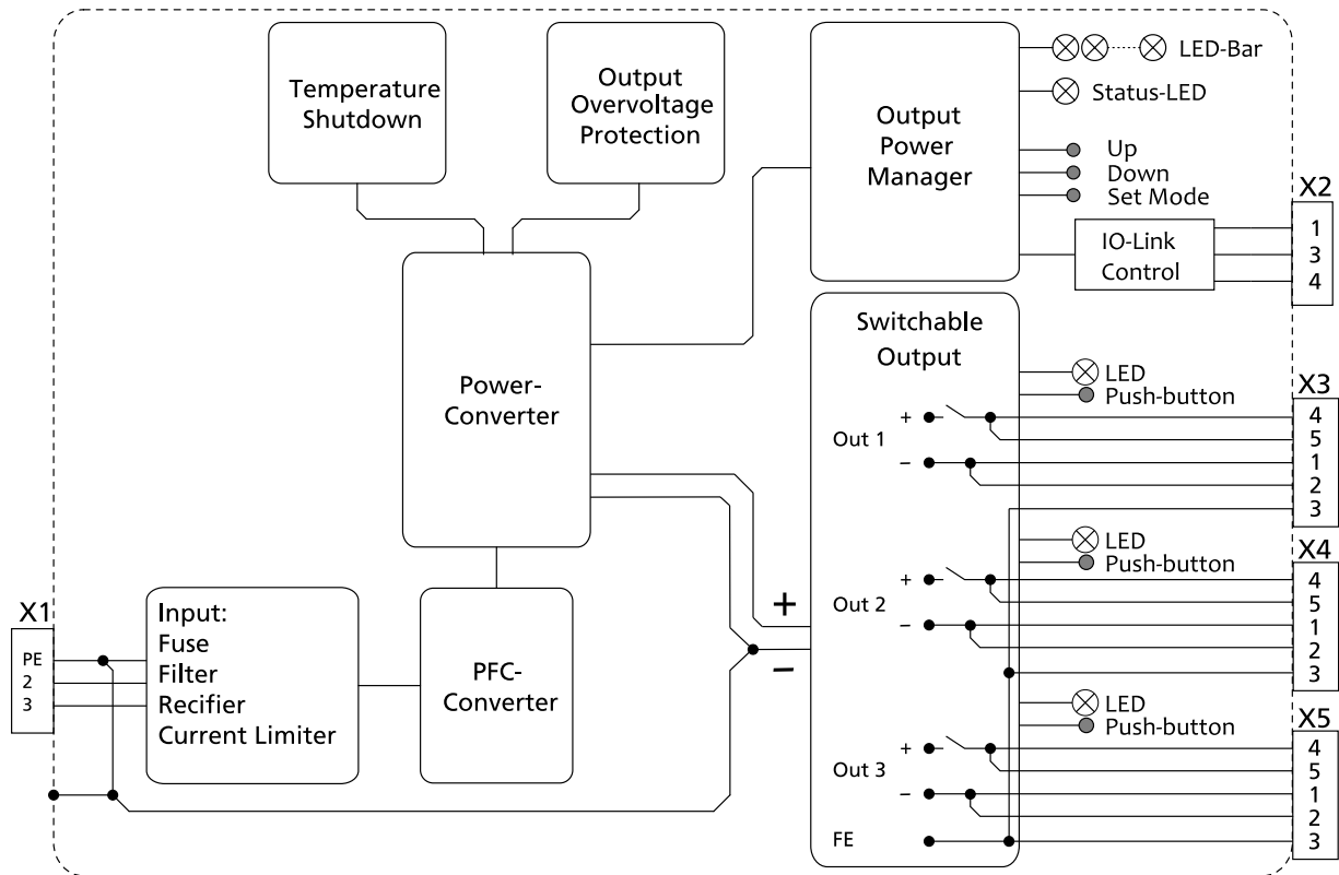
Fig. 12-1: Functional Diagram FPS300.246-073-156
