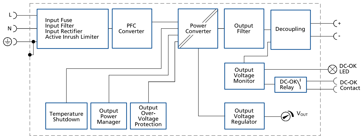
Fig. 12-1: Functional diagram
