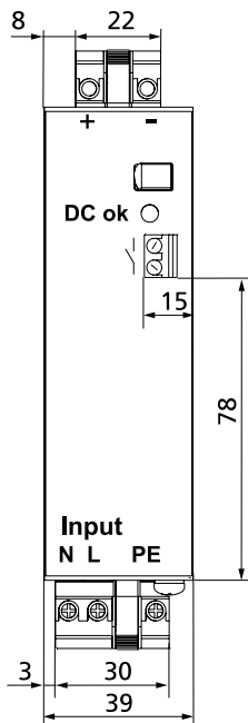
Fig. 23-1: Front view
