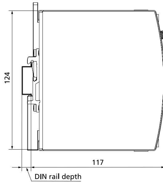
Fig. 23-2: Side view
