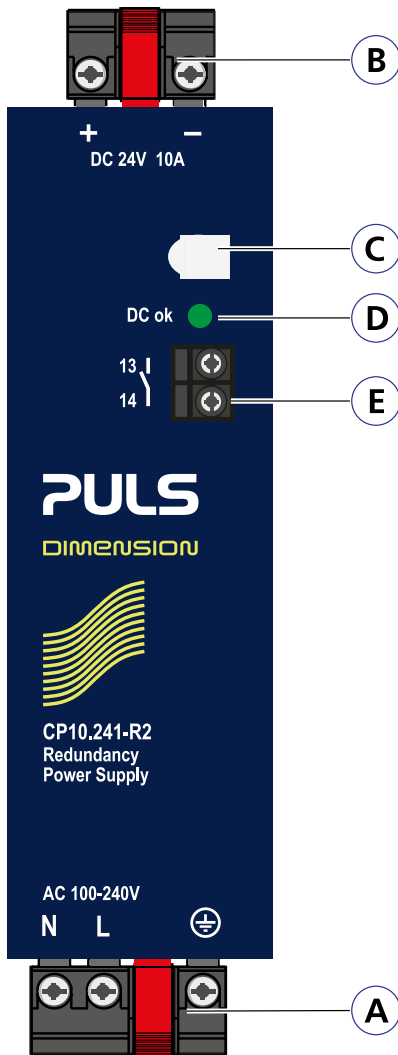
Fig. 15-1: Front side
