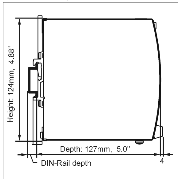
Fig. 16-2 Side view
