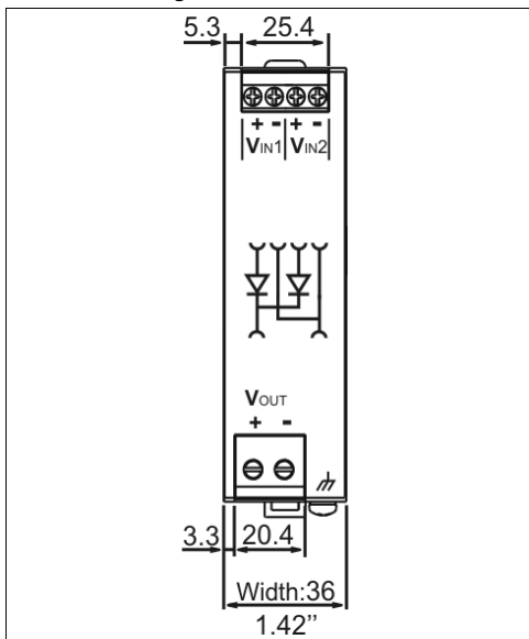
Fig. 16-1 Front view
