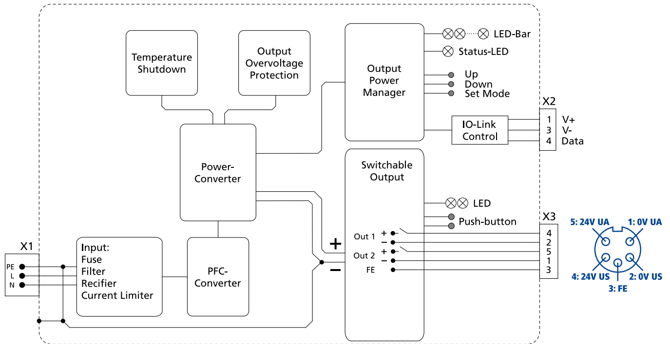
Fig. 12-1: Functional Diagram FPS300.245-016-101
