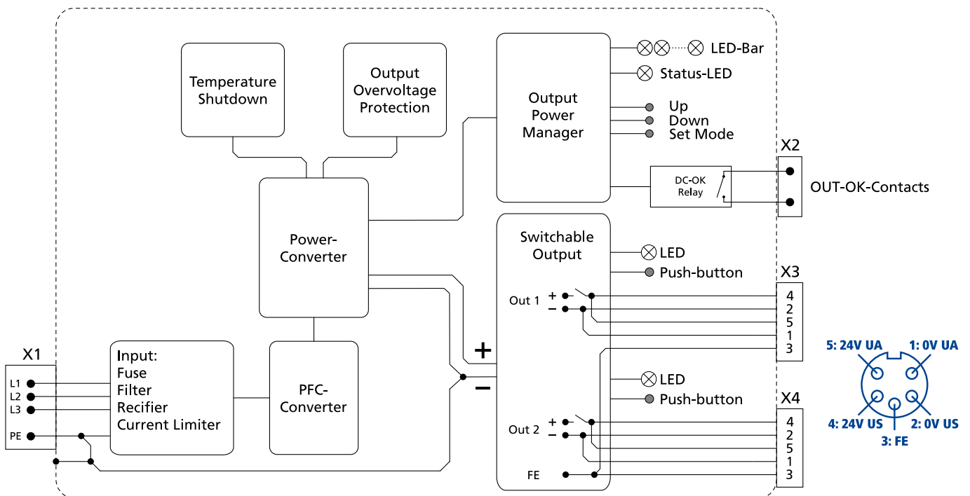
Fig. 12-2: Functional Diagram FPT500.245-053-113
