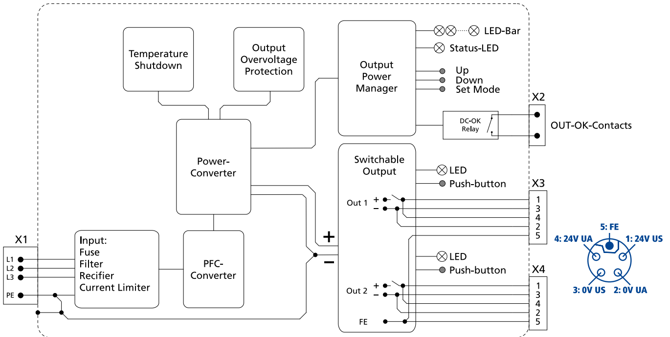
Fig. 12-1: Functional Diagram FPT500.245-034-106
