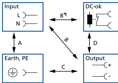
Fig. 19-1: Dielectric strength
