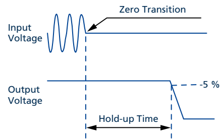
Fig. 7-2: Shut-down behaviour
