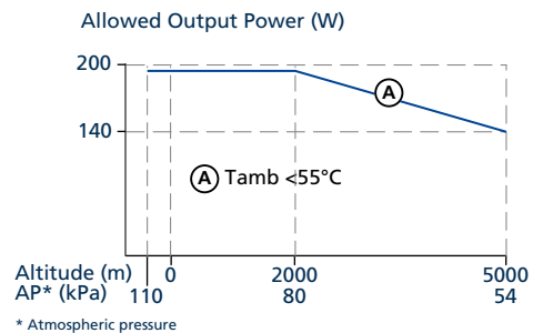
Fig. 16-2: Output power vs. altitude
