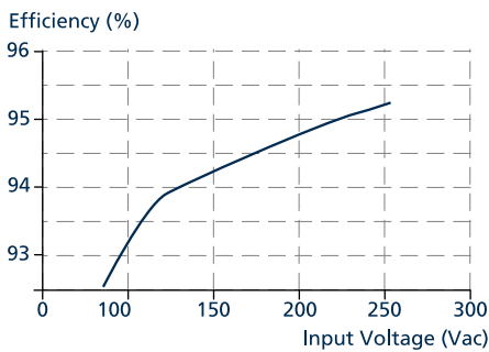
Fig. 10-3: Efficiency vs. input voltage at 24 V, 188 W, typ.
