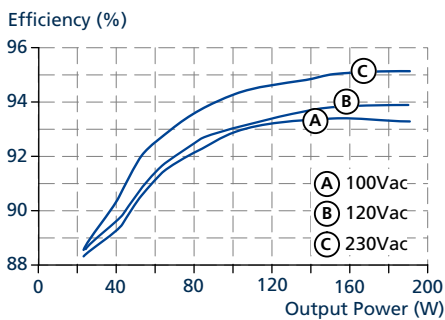
Fig. 10-1: Efficiency vs. output power at 24 V, typ.
