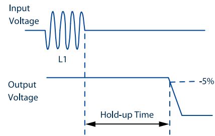
Fig. 8-2: Shut-down behaviour, definitions
