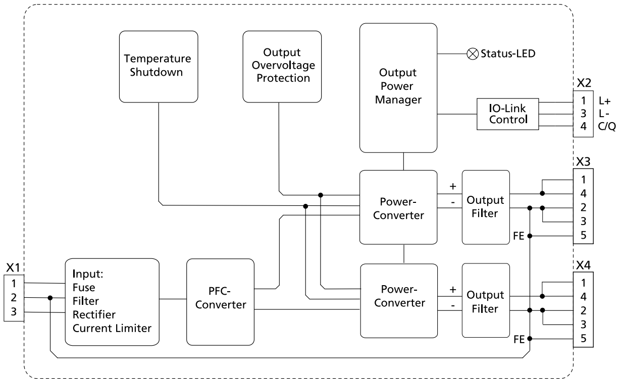
Fig. 13-1: Functional Diagram FPS202.242-004-IOL
