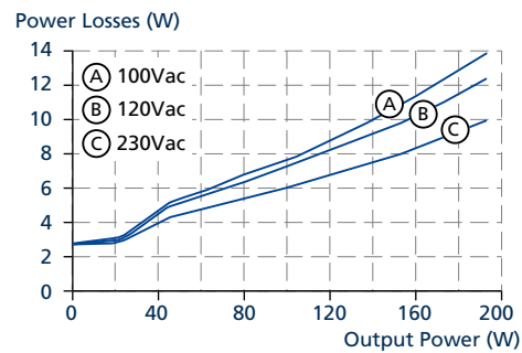
Fig. 10-2: Losses vs. output power at 24 V, typ.
