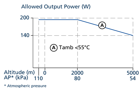
Fig. 17-2: Output power vs. altitude
