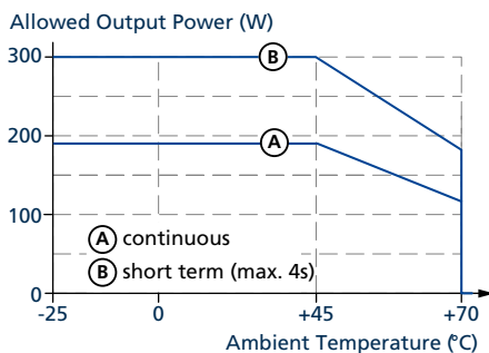
Fig. 17-1: Output power vs. ambient temp.
