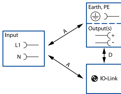
Fig. 19-1: Dielectric strength
