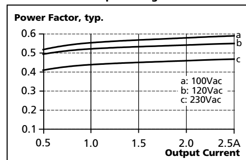
Fig. 3-4 Power factor vs. output load at 24V output voltage
