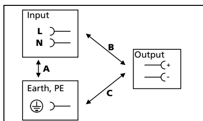
Fig. 17-1 Dielectric strength
