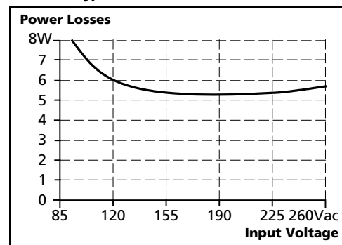
Fig. 8-4 Losses vs. input voltage at 24V, 2.5A, typ.
