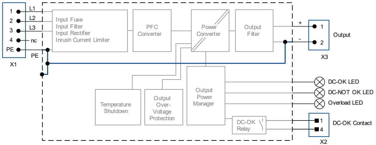
Fig. 12-1: Functional Diagram FPT300.242-008-102
