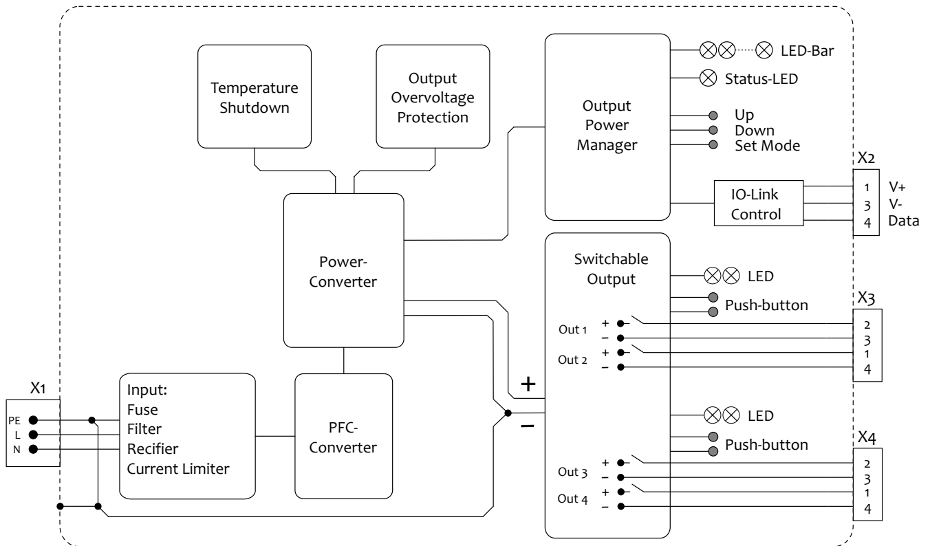
Fig. 12-1: Functional Diagram FPS300.245-047-103
