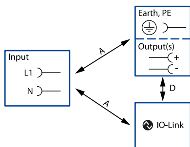
Fig. 17-1: Dielectric strength
