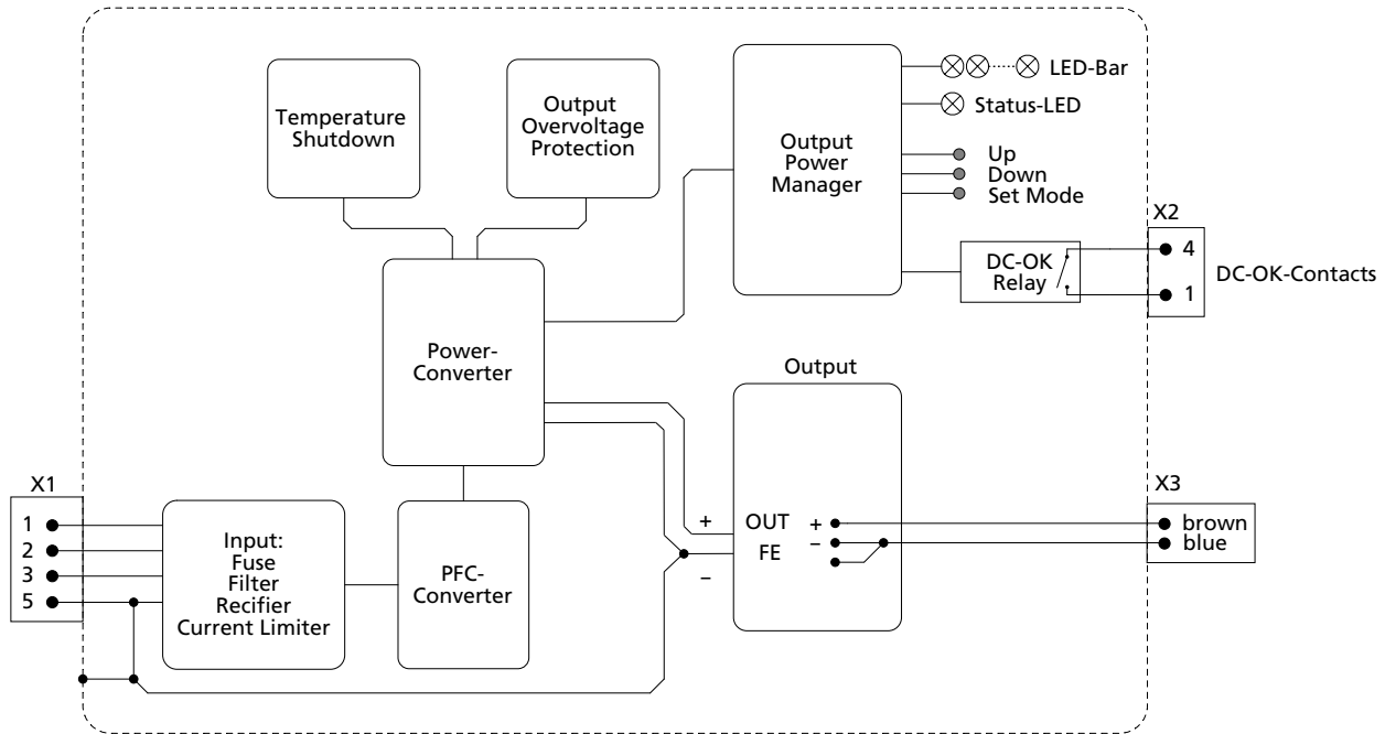
Fig. 12-1: Functional Diagram FPT500.241-006-113
