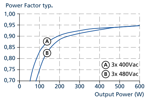
Fig. 3-4: Power factor vs. output power at 26 V output voltage
