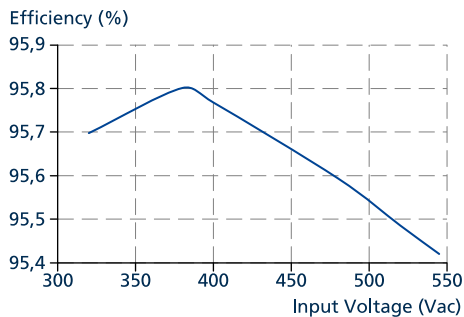
Fig. 9-3: Efficiency vs. input voltage at 26 V, 500 W, typ.
