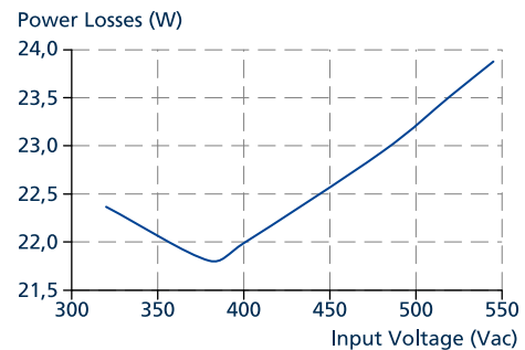
Fig. 9-4: Losses vs. input voltage at 26 V, 500 W, typ.
