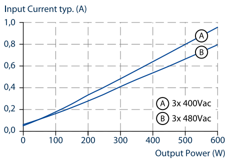
Fig. 3-3: Input current vs. output power at 26 V output voltage
