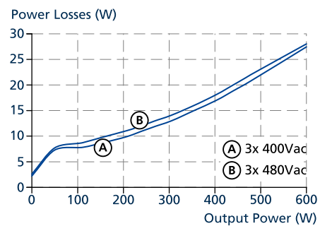
Fig. 9-2: Losses vs. output power at 26 V, typ.
