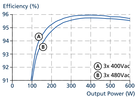
Fig. 9-1: Efficiency vs. output power at 26 V, typ.
