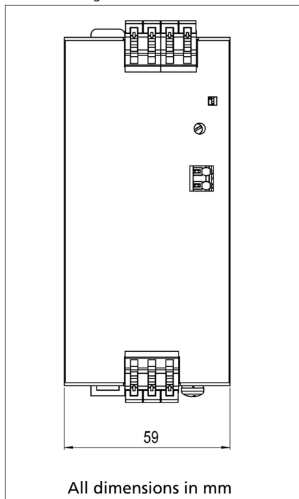
Fig. 21-1 Front view
