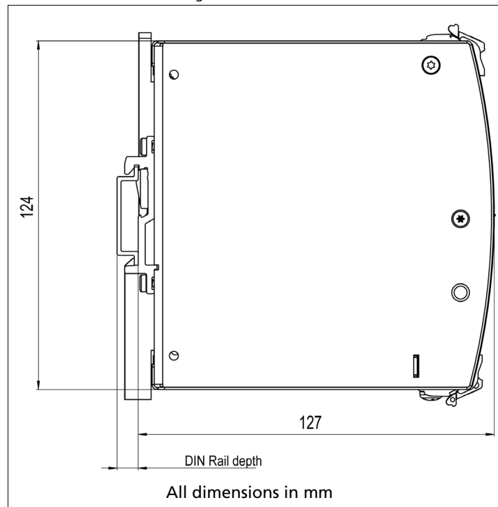
Fig. 21-2 Side view
