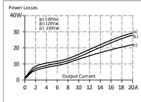
Fig. 9-2 Losses vs. output current at 24V, typ.
