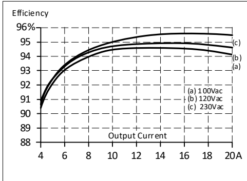
Fig. 9-1 Efficiency vs. output current at 24V, typ.
