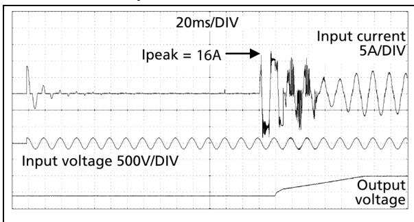
Fig. 5-1 Typical turn-on behaviour at nominal load, 120Vac input and +25°C ambient
