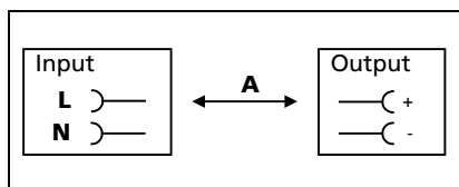
Fig. 17-1 Dielectric strength
