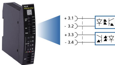
Fig. 11-1: Signaling interface using optocouplers
