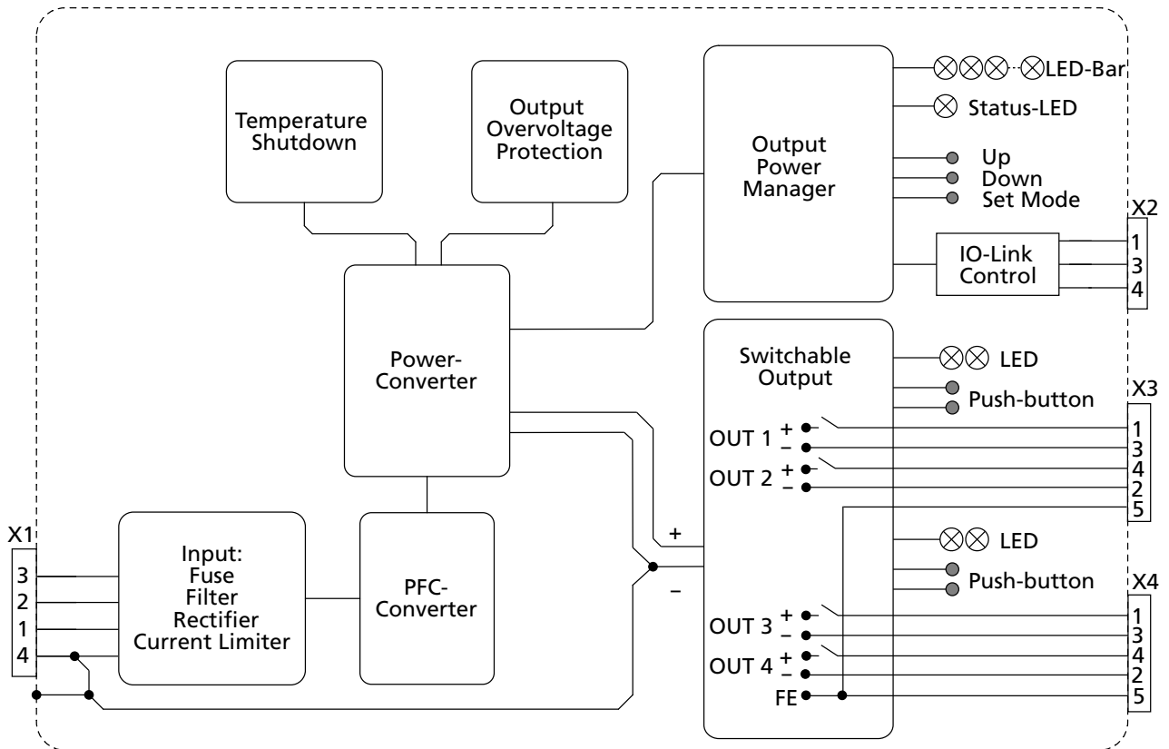
Fig. 12-1: Functional Diagram FPT500.245-070-161
