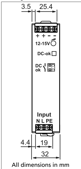
Fig. 21-1 Front view
